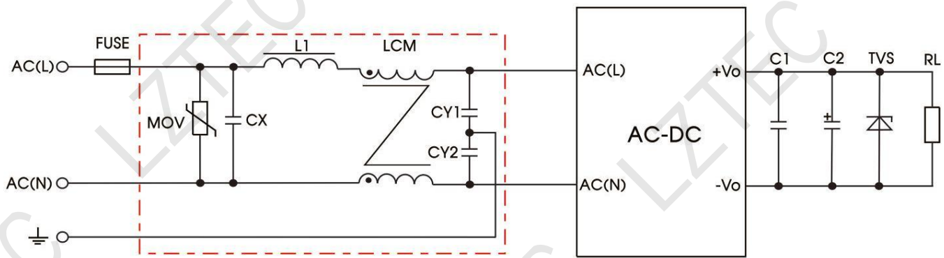
EMC recommended circuits
