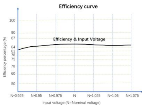
Figure 6: Efficiency VS Input Voltage (100% Load)
