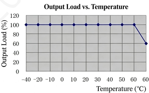
Operating Temperature Derating Curve
