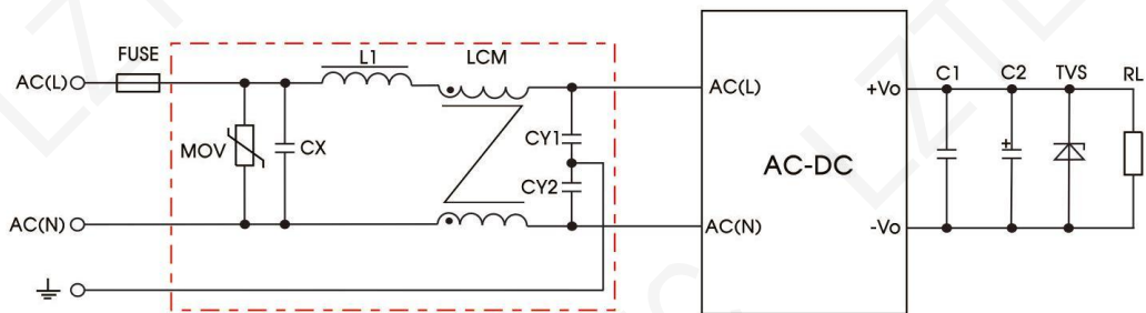
EMC Recommended Circuit
