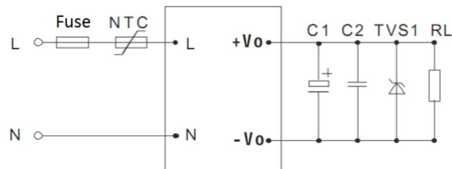
EMC Recommended Circuit
